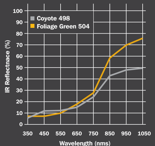
Solution-Dyed CORDURA® Fabric IR Reflectance
