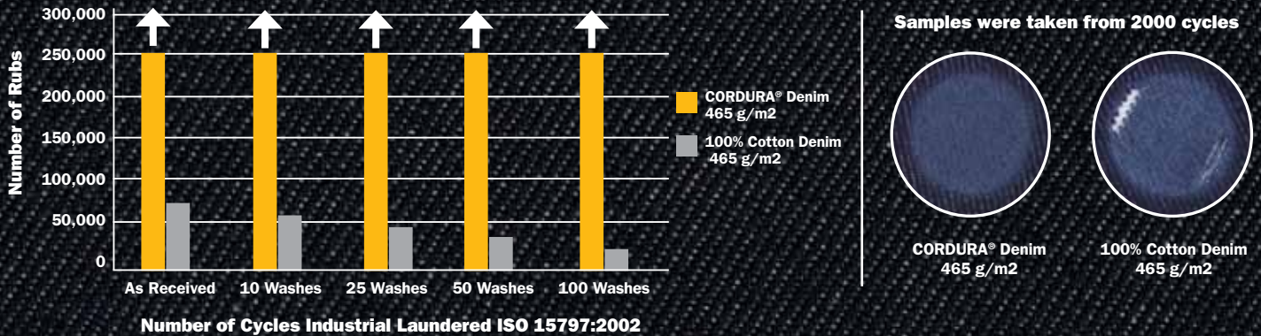
CORDURA ® Denim fabric vs 100% Cotton Denim fabric Martindale Abrasion BS EN ISO 12947-2:1999 Standard Woollen Abrasion with 12KPa weight Test stopped at 250,000 rubs
