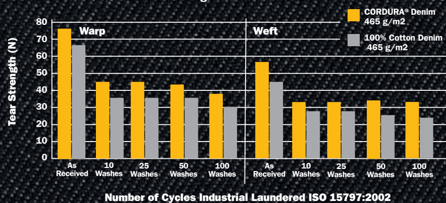
CORDURA ® Denim fabric vs 100% Cotton Denim fabric Tear Strength BS EN ISO 139347-2:2000
